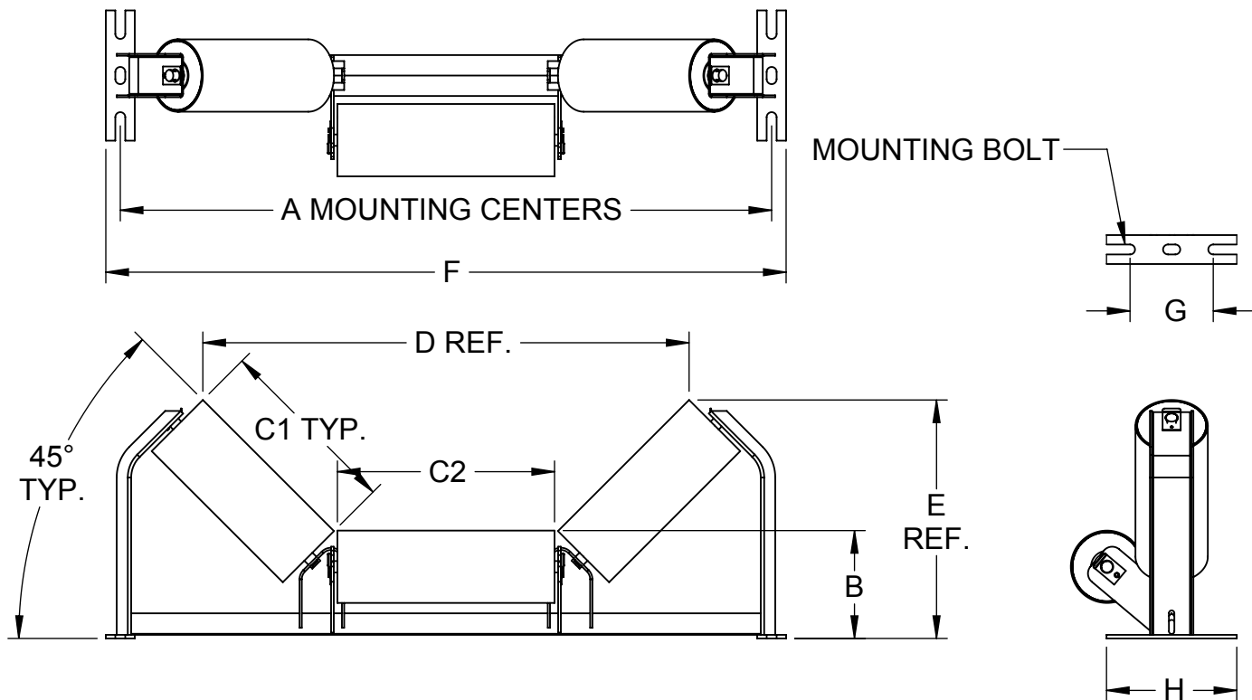
CEMA B 45° OFFSET CENTER ROLL TROUGH IDLER 4" DIAMETER ROLLS
