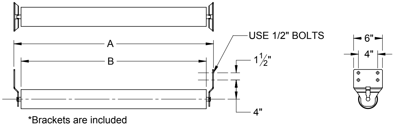
WEB MOUNT CHANNEL INSET RETURN IDLER 4" DIAMETER
