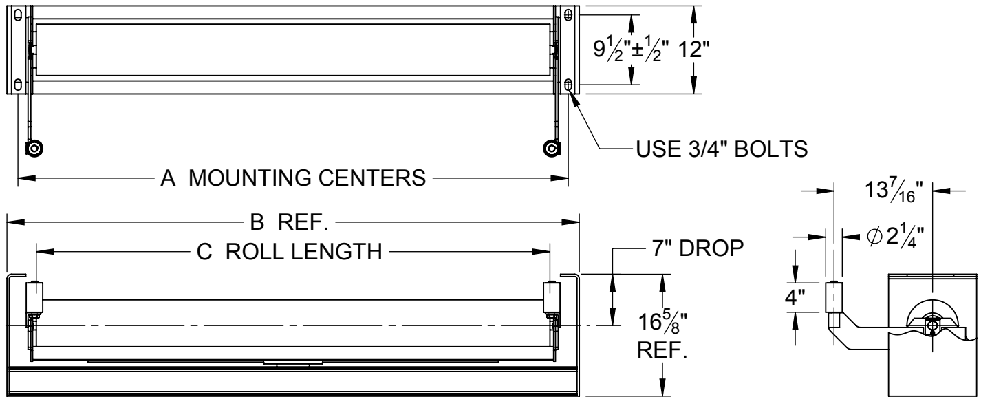
CEMA E SELF-ALIGNING RETURN IDLER 6" DIAMETER ROLLS
