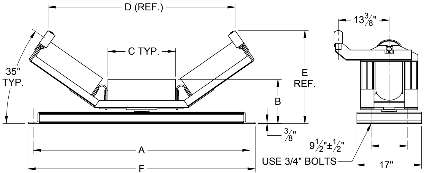
CEMA E 35° SELF-ALIGNING TROUGHING IDLER 6" DIAMETER ROLLS
